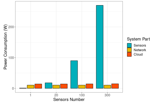
Fig. 8. End-to-end network energy consumption using sensors interval of 10s
