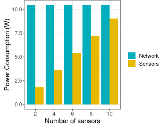
Fig. 4. Analysis of the variation of the number of sensors on the IoT/Network part energy consumption.
