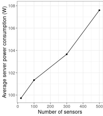
Fig. 6. Average server power consumption multiplied by the PUE (= 1.2) for sensors sending data every 10s
