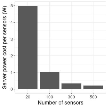
Fig. 7. Average sensors power cost on the server hosting only our VM with PUE (= 1.2) for sensors sending data every 10s
