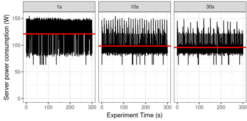
Fig. 8. Server energy consumption multiplied by the PUE (= 1.2) for 50 sensors sending requests at different transmission interval.
